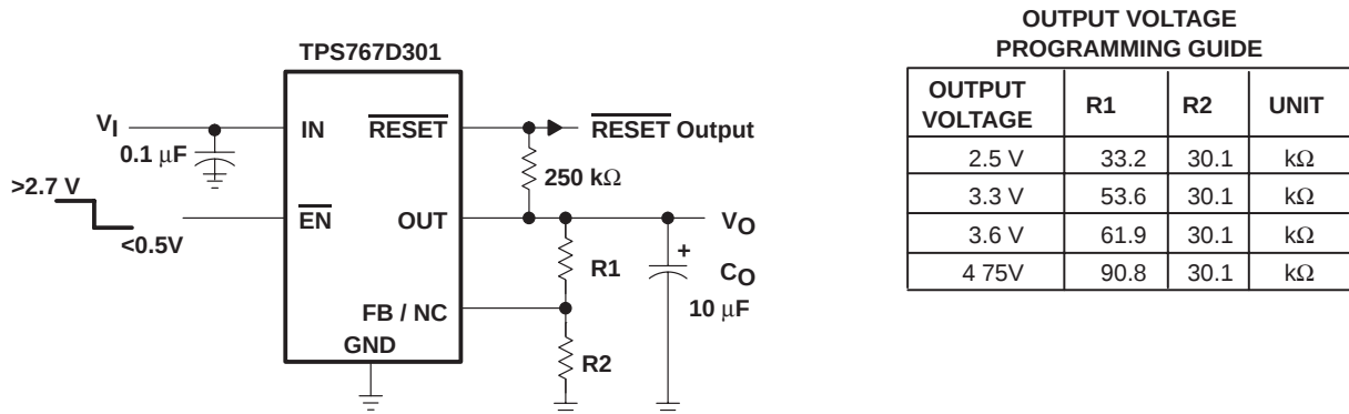
Figure 27. TPS767D301 Adjustable LDO Regulator Programming
